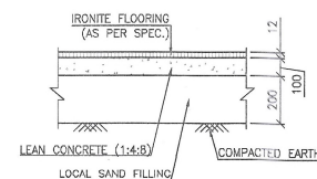
FLOORING DETAIL FOR STORE BUILDING
