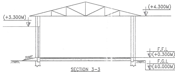
SECTION 3-3
