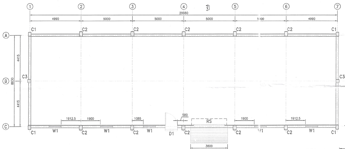
PLAN OF STORE BUILDING
