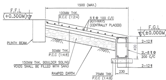
DETAIL OF RAMP
